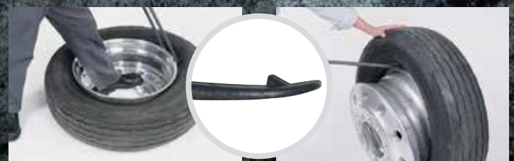
Demount end: Precision-forged angled tip slides between bead and rim easily. Forged design won't slip when demounting the second bead.
