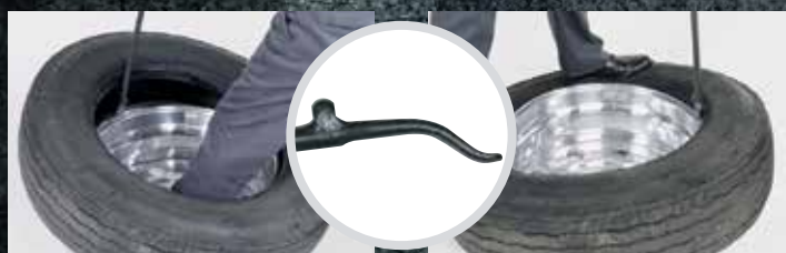
Mount end: Precision forged knob grips rim. New design won't slip during tire mounting. Special curve design always grabs the bead edge.
