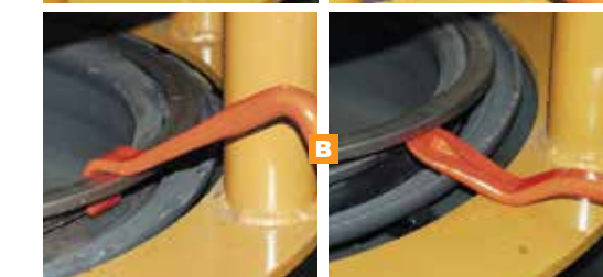
Mount end is used to mount split ring Demount end lifts and fully demounts split ring
